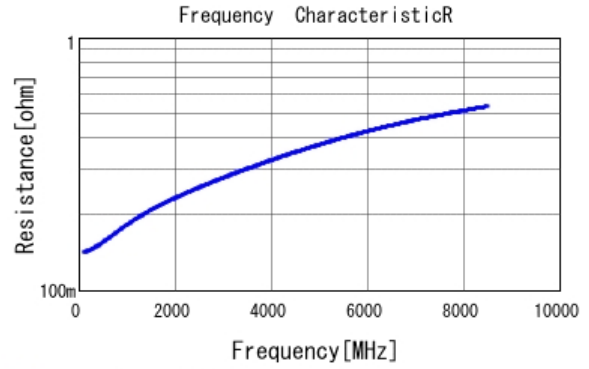
■ GRM0225C1H6R8WA03 R DCOV, 25degC
