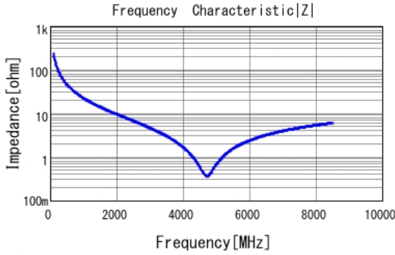
■ GRM0225C1H6R8WA03 |Z| DCOV, 25degC
