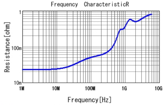
■ GRM2165C2A102JA01 R DCOV, 25degC
