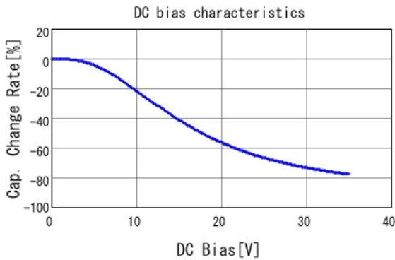
■ GRM219R7YA105KA12 C-DC bias capchange, 25.0degC, AC1.
