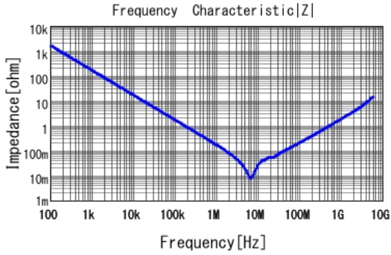
■ GRM219R7YA105KA12 |Z| DCOV, 25degC
