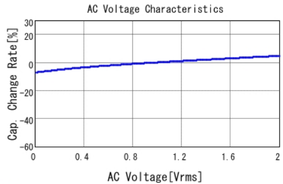
■ GRM219R7YA105KA12 C-AC Voltage capchange, DCOV, 25.0d
