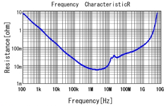
■ GRM219R7YA105KA12 R DCOV, 25degC
