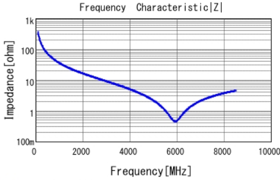
■ GRM0225C1H4R3WA03 |Z| DCOV, 25degC
