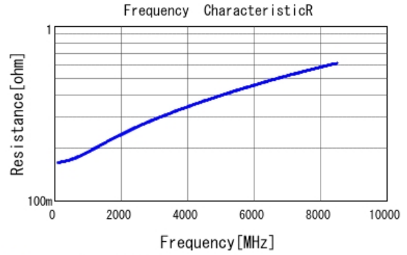
■ GRM0225C1H4R3WA03 R DCOV, 25degC
