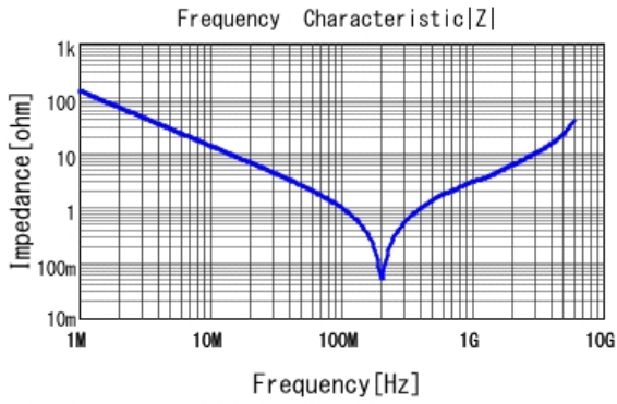
■ GRM2165C2A122JA01 |Z| DCOV, 25degC
