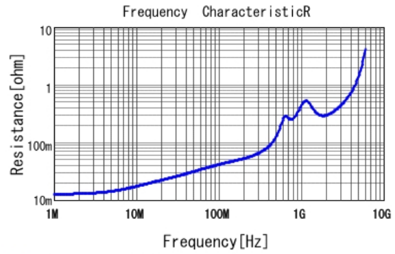
■ GRM2165C2A122JA01 R DCOV, 25degC
