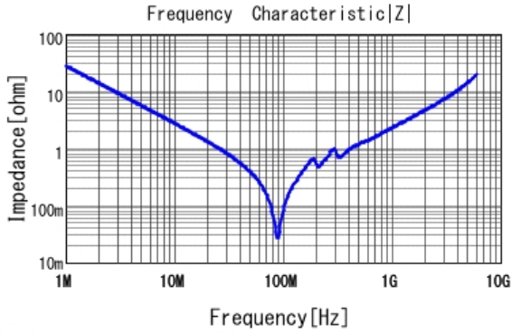
■ GRM2195C1H562JA01 |Z| DCOV, 25degC
