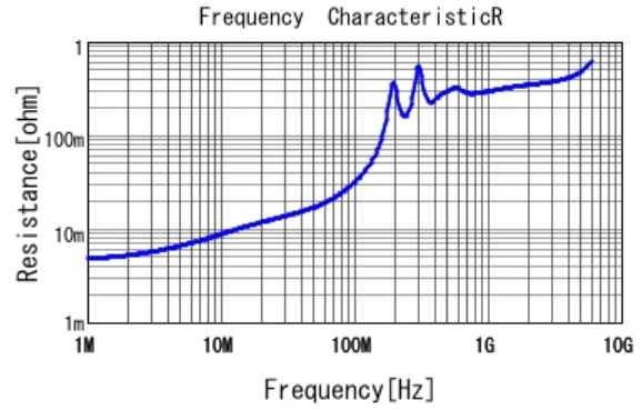
■ GRM2195C1H562JA01 R DCOV, 25degC
