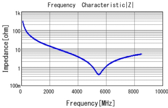
■ GRM0225C1H5R1WA03 |Z| DCOV, 25degC
