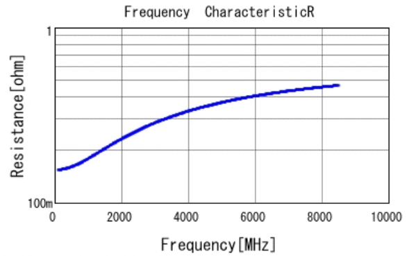
■ GRM0225C1H5R1WA03 R DCOV, 25degC
