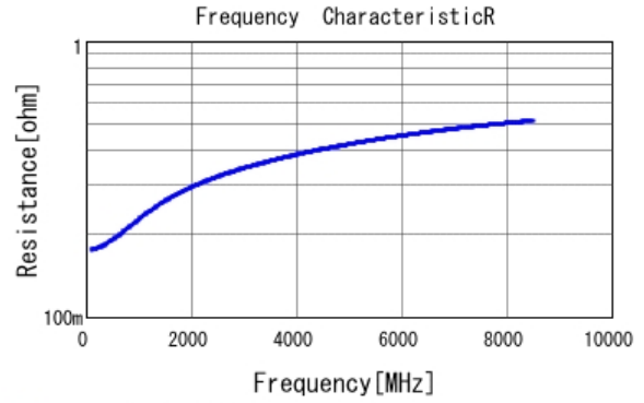
■ GRM0225C1H3R9WA03 R DCOV, 25degC
