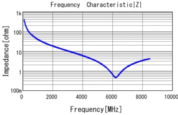
■ GRM0225C1H3R9WA03 |Z| DCOV, 25degC
