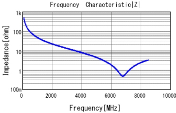
■ GRM0225C1H3R3WA03 |Z| DCOV, 25degC
