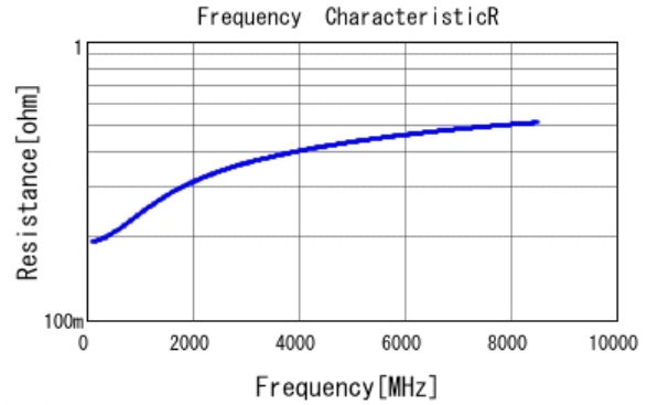
■ GRM0225C1H3R3WA03 R DCOV, 25degC
