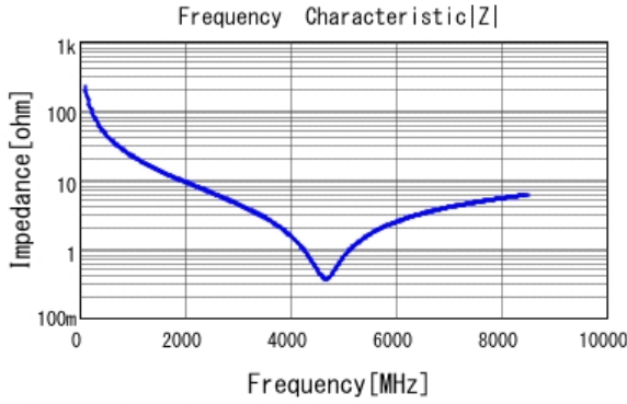
■ GRM0225C1H7R0WA03 |Z| DCOV, 25degC
