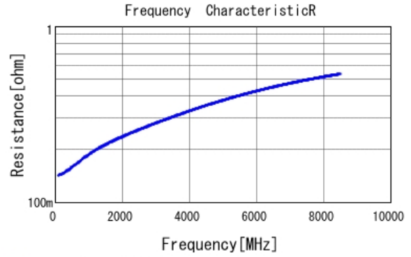
■ GRM0225C1H7R0WA03 R DCOV, 25degC
