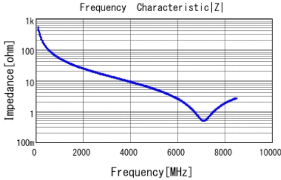
■ GRM0225C1H3R0WA03 |Z| DCOV, 25degC
