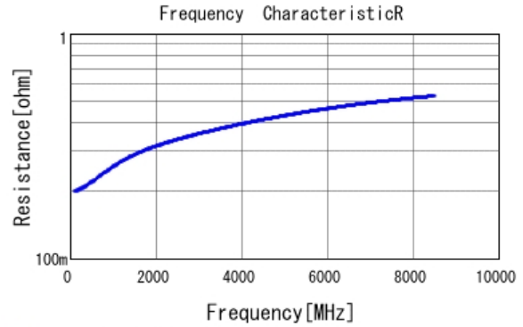
■ GRM0225C1H3R0WA03 R DCOV, 25degC
