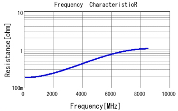
■ GRM0225C1H300GA02 R DCOV, 25degC
