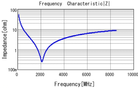
■ GRM0225C1H300GA02 |Z| DCOV, 25degC
