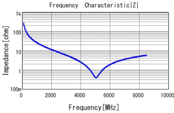
■ GRM0225C1H5R9DA03 |Z| DC0V, 25degC
