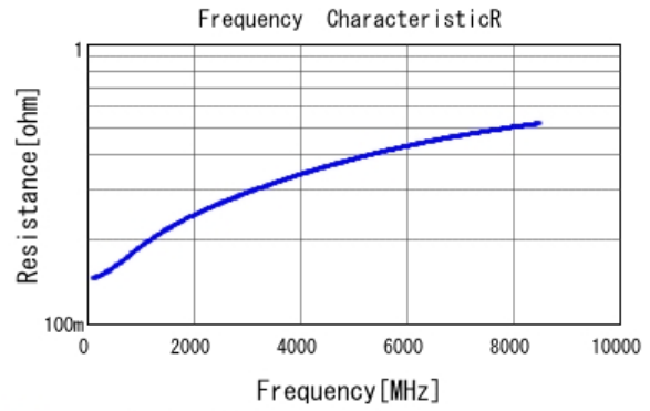
■ GRM0225C1H5R9DA03 R DC0V, 25degC
