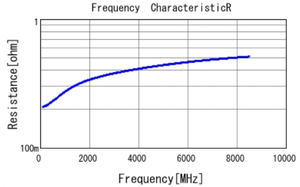
■ GRM0225C1H2R7WA03 R DCOV, 25degC
