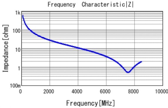
■ GRM0225C1H2R7WA03 |Z| DCOV, 25degC
