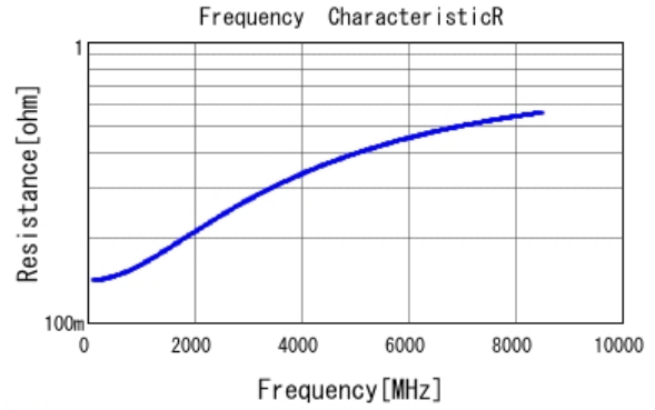
■ GRM0225C1H7R1CA03 R DCOV, 25degC
