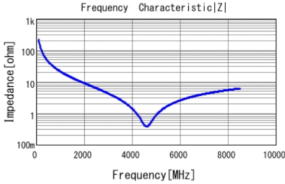
■ GRM0225C1H7R1CA03 |Z| DCOV, 25degC
