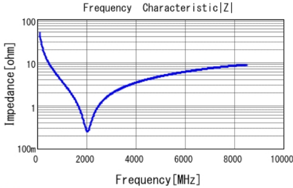
■ GRM0225C1H330JA02 |Z| DCOV, 25degC
