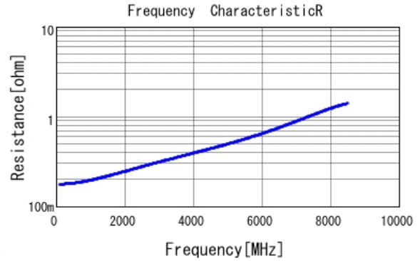
■ GRM0225C1H330JA02 R DCOV, 25degC
