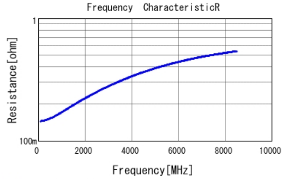
■ GRM0225C1H6R2WA03 R DCOV, 25degC
