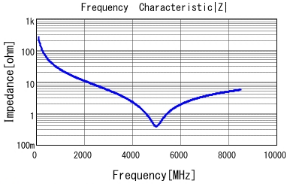
■ GRM0225C1H6R2WA03 |Z| DCOV, 25degC
