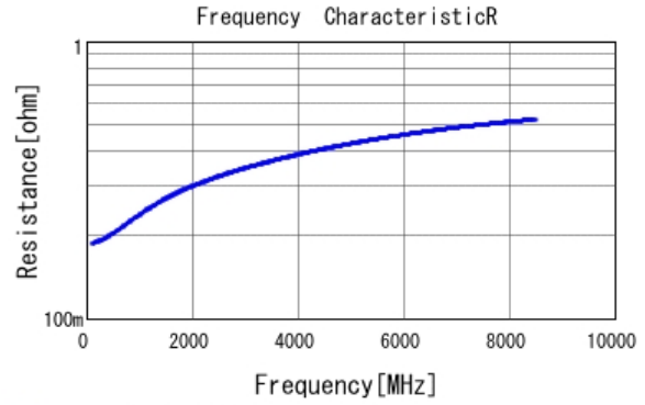
■ GRM0225C1H3R6WA03 R DCOV, 25degC
