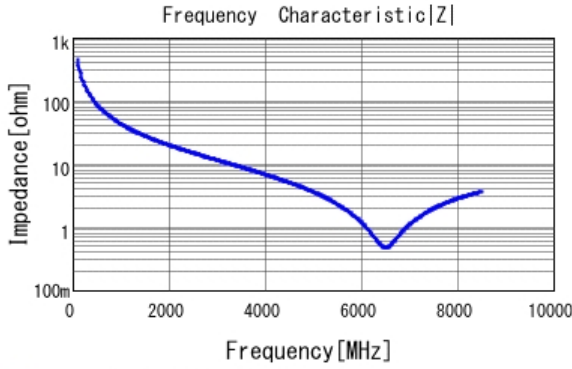
■ GRM0225C1H3R6WA03 |Z| DCOV, 25degC
