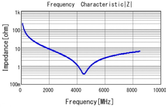
■ GRM0225C1H7R5WA03 |Z| DC0V, 25degC
