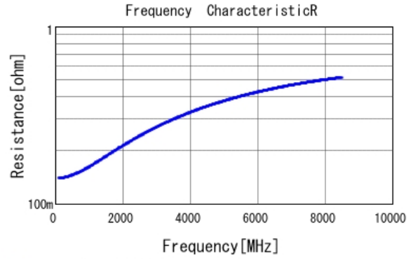
■ GRM0225C1H7R5WA03 R DC0V, 25degC
