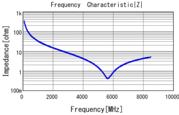
■ GRM0225C1H4R7WA03 |Z| DCOV, 25degC
