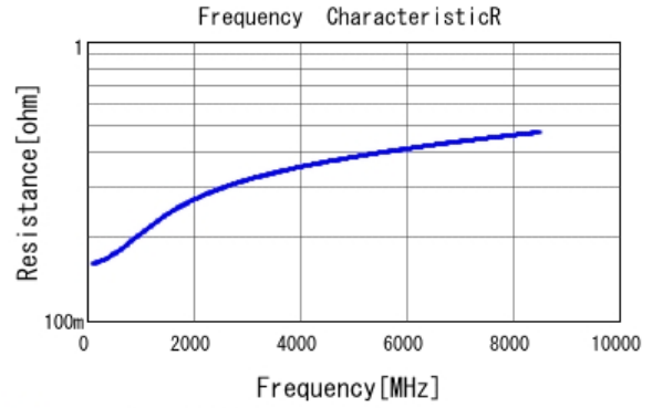
■ GRM0225C1H4R7WA03 R DCOV, 25degC
