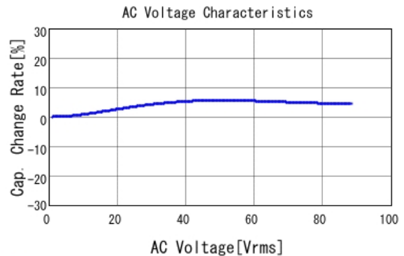
GCM21A7U2E101JX01 C-AC Voltage capchange, DC0V, 25.0d
