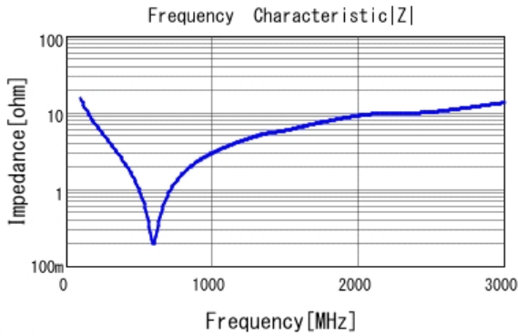
GCM21A7U2E101JX01 |Z| DC0V, 25degC
