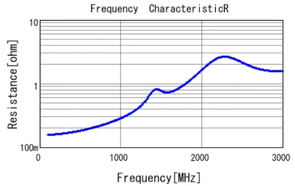
GCM21A7U2E101JX01 R DC0V, 25degC
