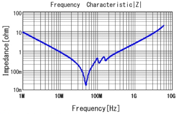
GCM21B5C1H183JA16 |Z| DCOV, 25degC
