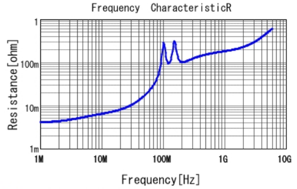
GCM21B5C1H183JA16 R DCOV, 25degC
