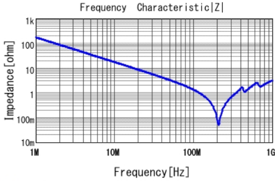
■ GCM21B5C2J102JX03 |Z| DC0V, 25degC
