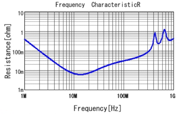
■ GCM21B5C2J102JX03 R DC0V, 25degC
