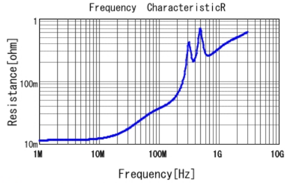
GCM21A7U2E222JX01 R DC0V, 25degC
