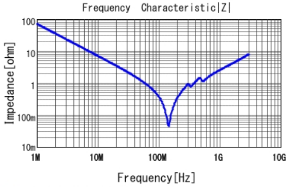
GCM21A7U2E222JX01 |Z| DC0V, 25degC
