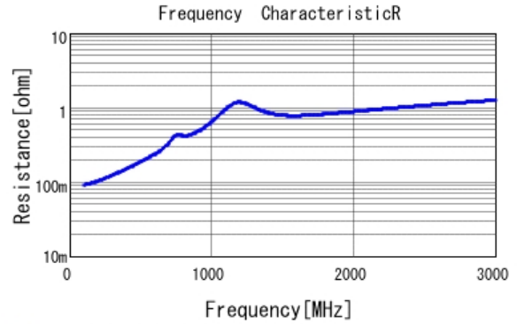
■ GCM21A7U2E331JX01 R DC0V, 25degC
