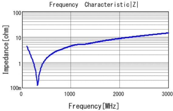
■ GCM21A7U2E331JX01 |Z| DC0V, 25degC
