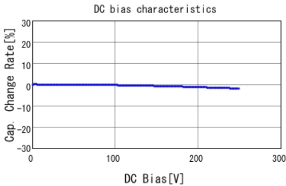
■ GCM21A7U2E331JX01 C-DC bias capchange, 25.0degC, AC1V
