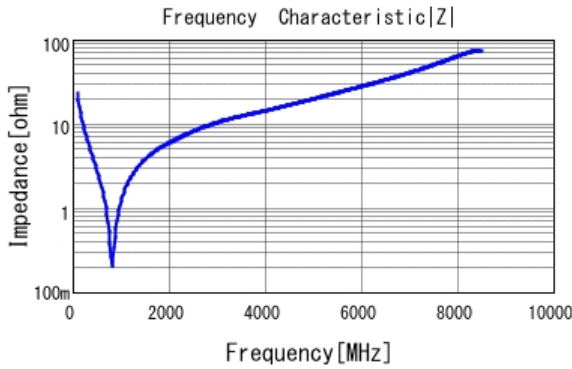
■ GCM1885C2A680JA16 |Z| DCOV, 25degC
