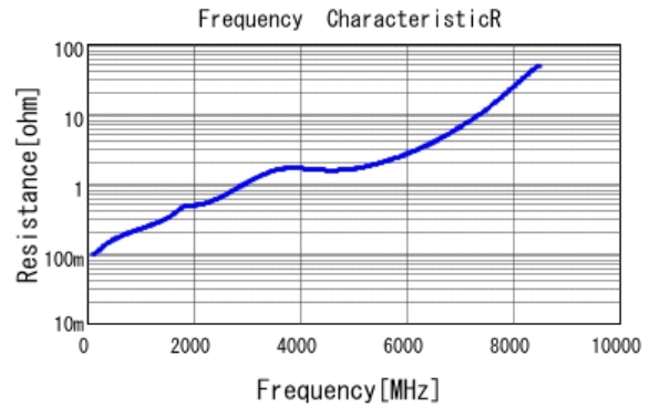
■ GCM1885C2A680JA16 R DCOV, 25degC
