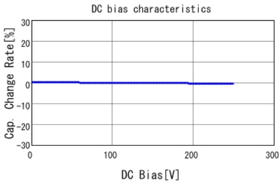
■ GCM21A7U2E271JX01 C-DC bias capchange, 25.0degC, AC1V
