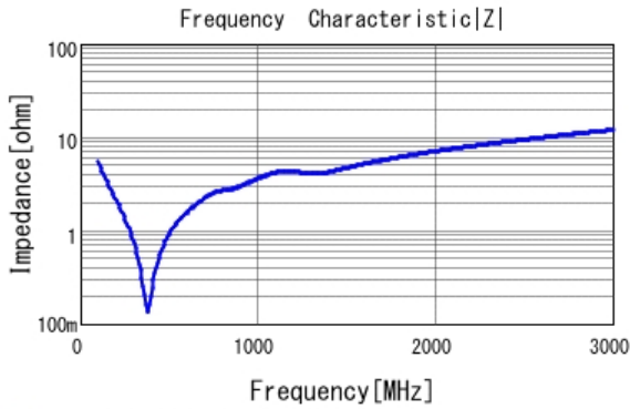
■ GCM21A7U2E271JX01 |Z| DC0V, 25degC
