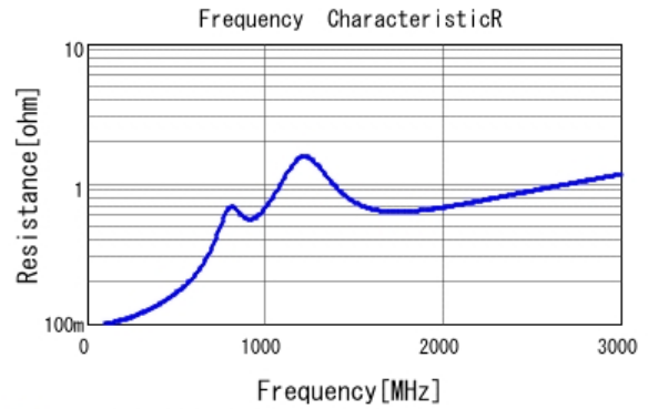
■ GCM21A7U2E271JX01 R DC0V, 25degC
