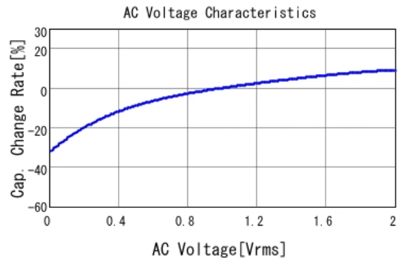
■ GCM21BC71A475KA73 C-AC Voltage capchange, DC0V, 25.0d
