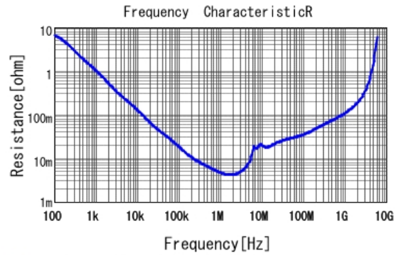
■ GCM21BC71A475KA73 R DC0V, 25degC
