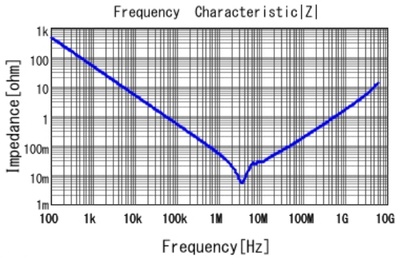
■ GCM21BC71A475KA73 |Z| DC0V, 25degC
