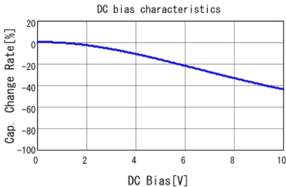
■ GCM21BC71A475KA73 C-DC bias capchange, 25.0degC, AC1.
