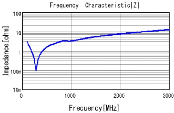
■ GCM21A7U2E471JX01 |Z| DC0V, 25degC
