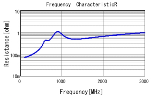
■ GCM21A7U2E471JX01 R DC0V, 25degC
