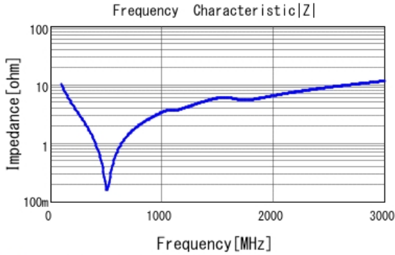
■ GCM21A7U2E151JX01 |Z| DC0V, 25degC
