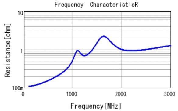
■ GCM21A7U2E151JX01 R DC0V, 25degC
