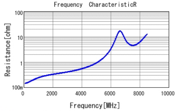
■ GCM1885C2A5R0CA16 R DCOV, 25degC
