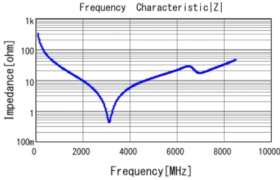
■ GCM1885C2A5R0CA16 |Z| DCOV, 25degC
