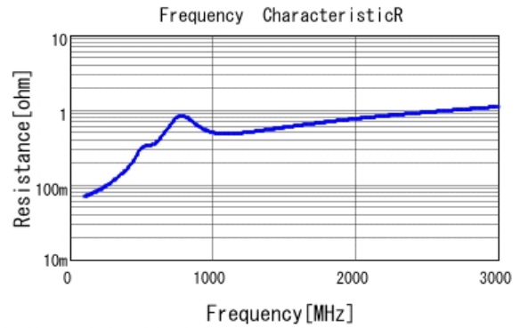
■ GCM21A7U2E681JX01 R DC0V, 25degC
