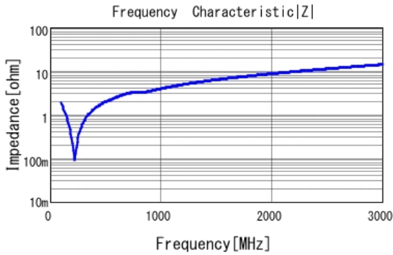
■ GCM21A7U2E681JX01 |Z| DC0V, 25degC
