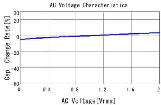
GCM219R71E474KA55 C-AC Voltage capchange, DCOV, 25.0d
