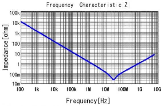
■ GRM033R61E224KE01 |Z| DCOV, 25degC
