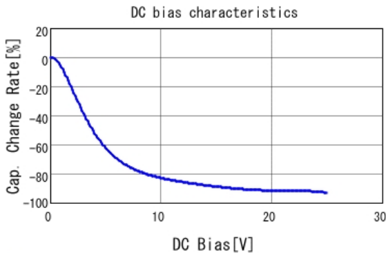
■ GRM033R61E224KE01 C-DC bias capchange, 25.0degC, AC1V
