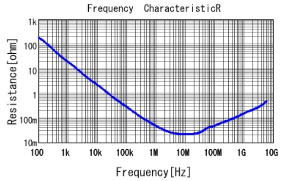
■ GRM033R61E224KE01 R DCOV, 25degC
