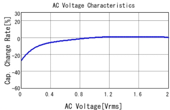
■ GRM033R61E224KE01 C-AC Voltage capchange, DCOV, 25.0d
