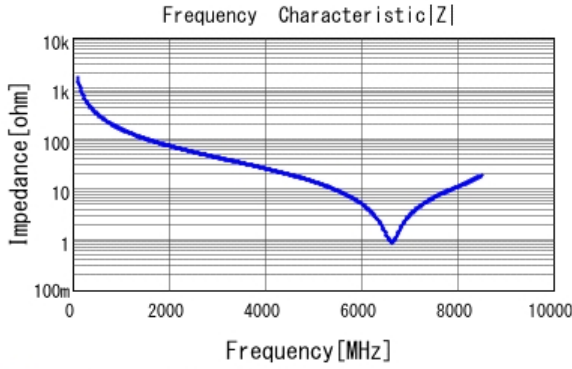
■ GCM1885C2A1R0CA16 |Z| DCOV, 25degC
