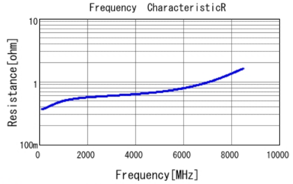
■ GCM1885C2A1R0CA16 R DCOV, 25degC
