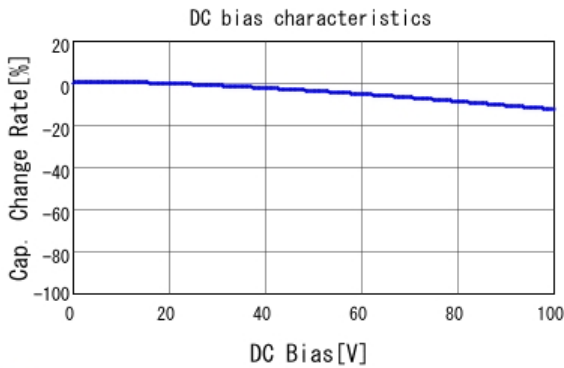
GCM2199E2A152KA05 C-DC bias capchange, 20.0degC, AC1V
