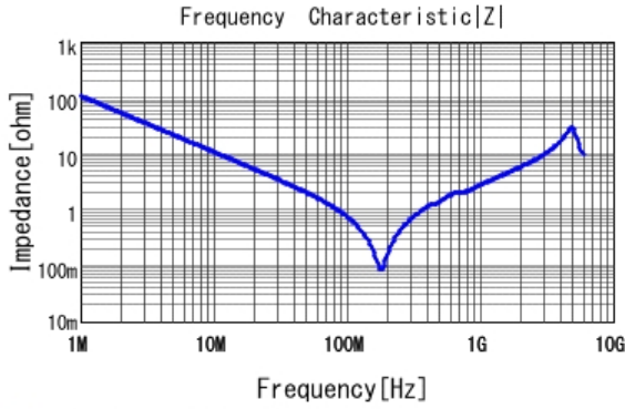
GCM2199E2A152KA05 |Z| DC0V, 20degC
