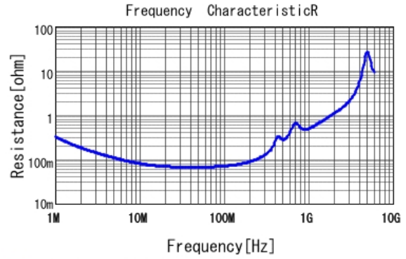
GCM2199E2A152KA05 R DC0V, 20degC
