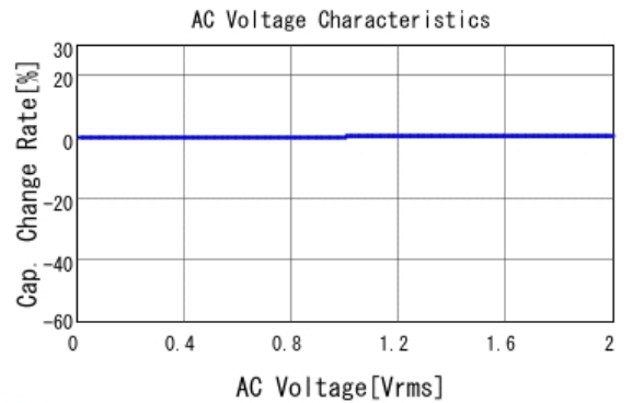
GCM2199E2A152KA05 C-AC Voltage capchange, DC0V, 20.0d
