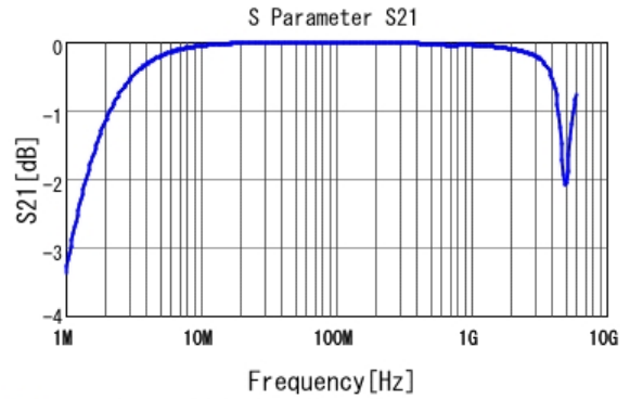
■ GCM2199E2A152KA05 S21 DC0V, 20degC
