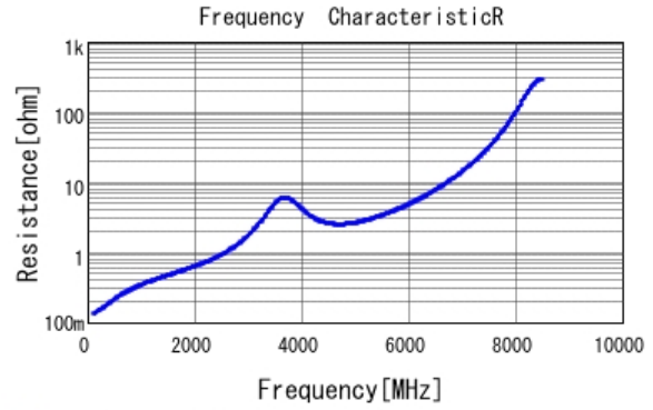
■ GCM1885C2A180JA16 R DCOV, 25degC
