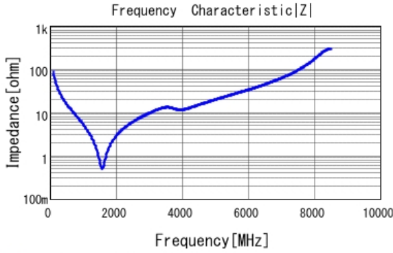
■ GCM1885C2A180JA16 |Z| DCOV, 25degC
