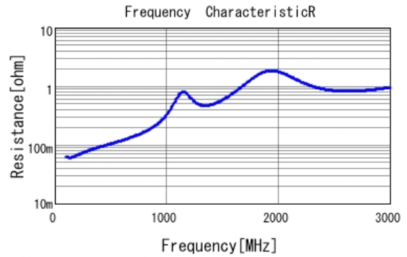
■ GCM21A5C2E221JX01 R DC0V, 25degC
