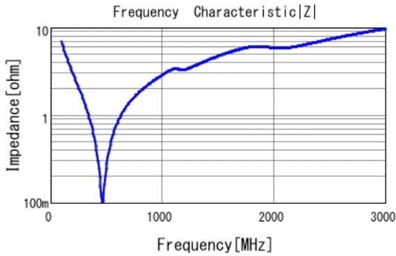
■ GCM21A5C2E221JX01 |Z| DC0V, 25degC
