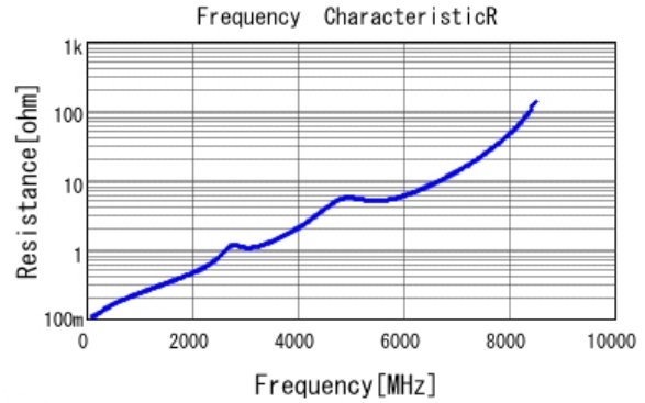
■ GCM1885C2A270JA16 R DCOV, 25degC
