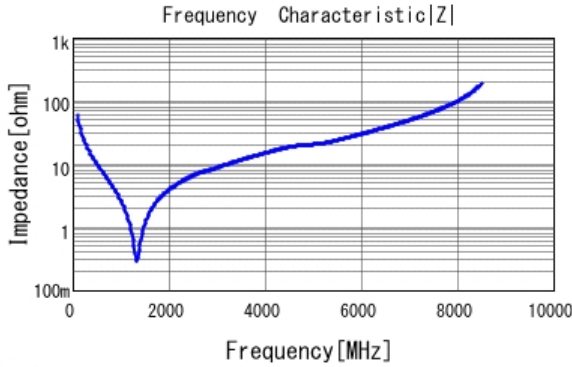
■ GCM1885C2A270JA16 |Z| DCOV, 25degC
