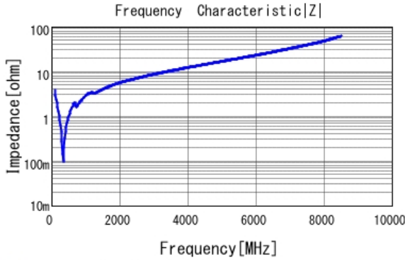
■ GCM1885C2A391JA16 |Z| DCOV, 25degC
