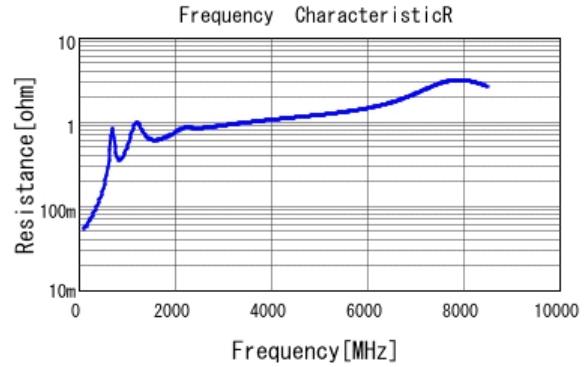
■ GCM1885C2A391JA16 R DCOV, 25degC
