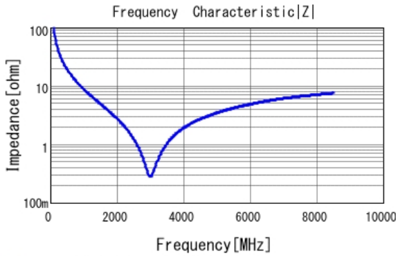
■ GRM0225C1E160GA03 |Z| DCOV, 25degC
