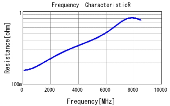
■ GRM0225C1E160GA03 R DCOV, 25degC
