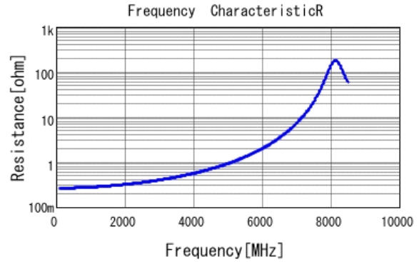
■ GCM1885C2A3R3CA16 R DCOV, 25degC
