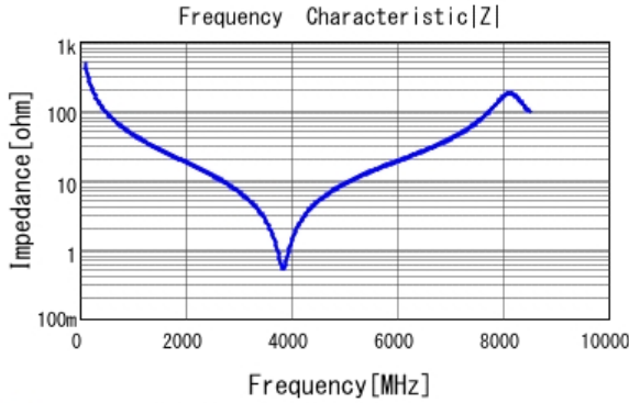
■ GCM1885C2A3R3CA16 |Z| DCOV, 25degC
