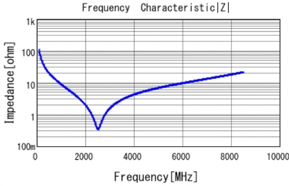
■ GRM0335C1H150GA01 |Z| DCOV, 25degC
