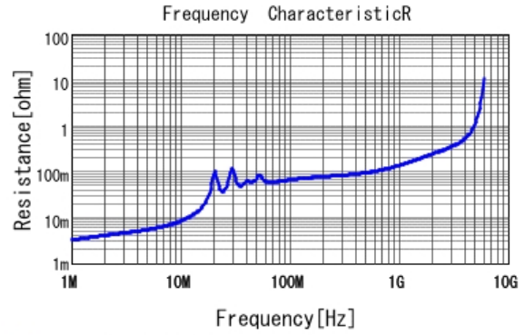
■ GRM31C5C1H224JE02 R DCOV, 25degC
