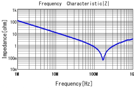
GCM21A5C2E152JX01 |Z| DC0V, 25degC
