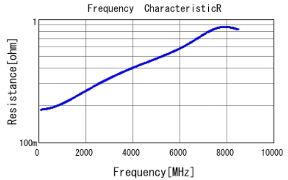
■ GRM0225C1E200GA02 R DCOV, 25degC
