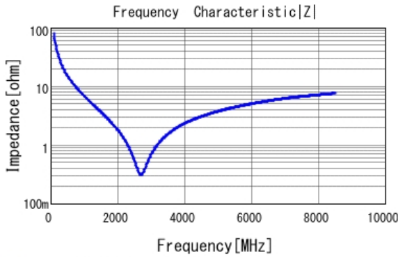
■ GRM0225C1E200GA02 |Z| DCOV, 25degC
