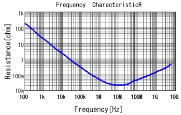
■ GRM033R61E224ME01 R DCOV, 25degC
