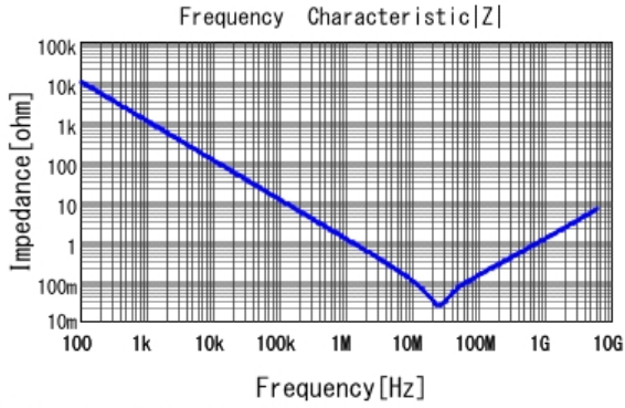
■ GRM033R61E224ME01 |Z| DCOV, 25degC
