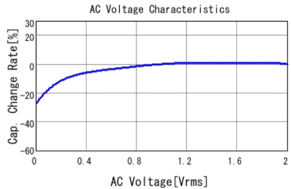
■ GRM033R61E224ME01 C-AC Voltage capchange, DCOV, 25.0d
