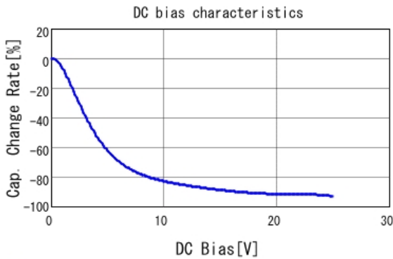
■ GRM033R61E224ME01 C-DC bias capchange, 25.0degC, AC1V
