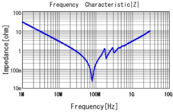
■ GCM32B7U2J562JX01 |Z| DC0V, 25degC
