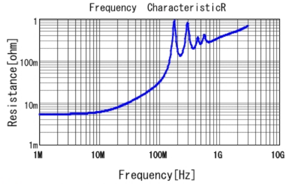
■ GCM32B7U2J562JX01 R DC0V, 25degC
