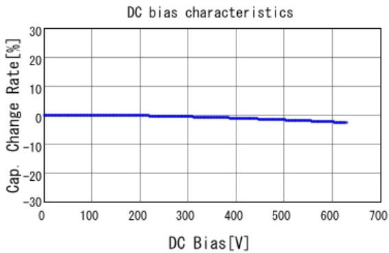
■ GCM32B7U2J562JX01 C-DC bias capchange, 25.0degC, AC1V
