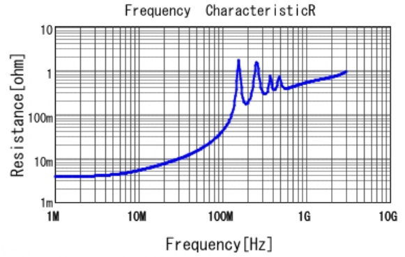
■ GCM43D7U3A472JX01 R DC0V, 25degC
