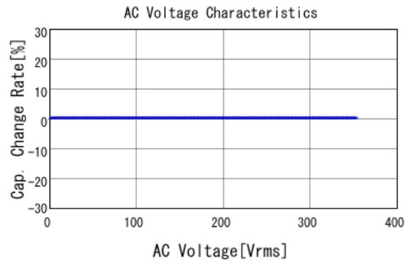
■ GCM43D7U3A472JX01 C-AC Voltage capchange, DC0V, 25.0d
