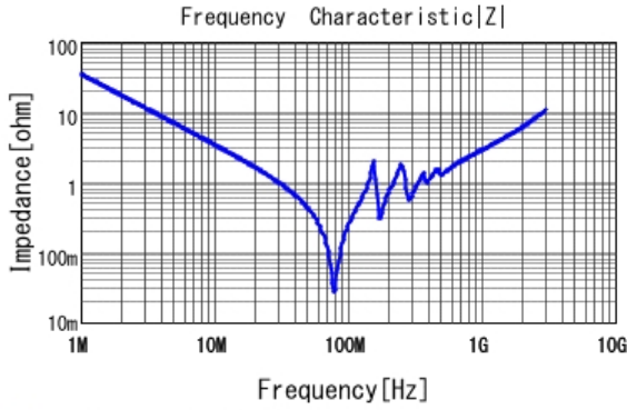
■ GCM43D7U3A472JX01 |Z| DC0V, 25degC
