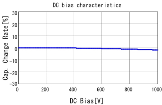
■ GCM43D7U3A472JX01 C-DC bias capchange, 25.0degC, AC1V
