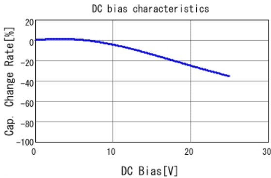
■ GCM31ML81E105KA37 C-DC bias capchange, 25.0degC, AC1.
