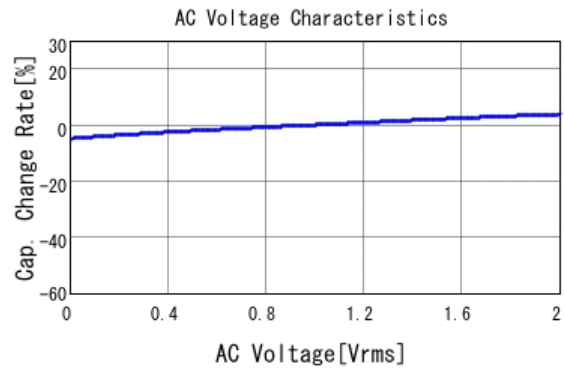
■ GCM31ML81E105KA37 C-AC Voltage capchange, DCOV, 25.0d
