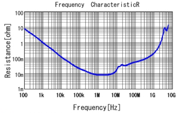
■ GCM31ML81E105KA37 R DCOV, 25degC
