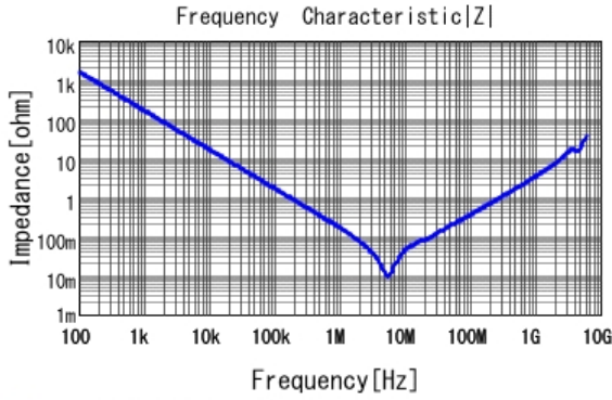
■ GCM31ML81E105KA37 |Z| DCOV, 25degC
